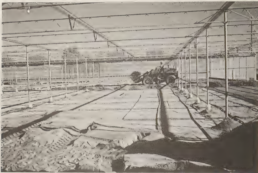
FIGURE 8.4 Back filling with 12 in. of sand.
