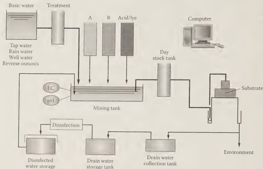
FIGURE 3.18 Overview of a complete disinfection-injection-irrigation system. (Adapted from K. Welleman, The Netherlands. 6th Curso Y Congreso Internacional de Hidroponia en Mexico . Toluca, Mexico, April 17–19, 2008a. With permission. Courtesy of George Barile, Accurate Art, Inc., Holbrook, NY.)
