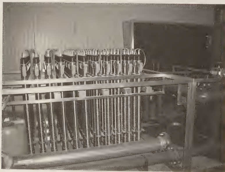
FIGURE 10.30 UV sterilizers on return solution. (From Eurofresh Farms, Wilcox, AZ. With permission.)
