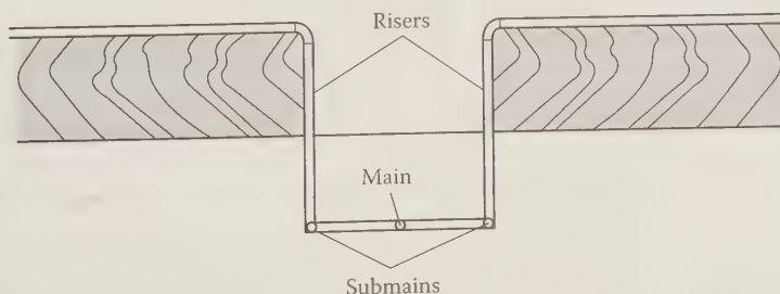
FIGURE 9.14 Main header with submain headers placed underground. (Courtesy of George Barile, Accurate Art, Inc., Holbrook, NY.)
