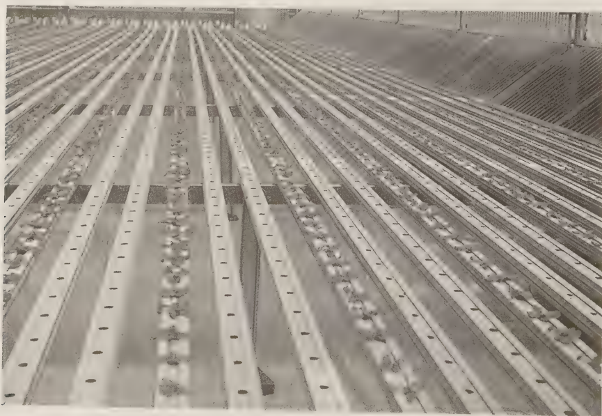
FIGURE 6.18 NFT channels raised about 3 ft by a metal frame. Note: The convection tubes underneath the table and the cooling pad behind the deflector panels at the upper right. (From F.W. Armstrong Ranch, Oak View, CA. With permission.)
