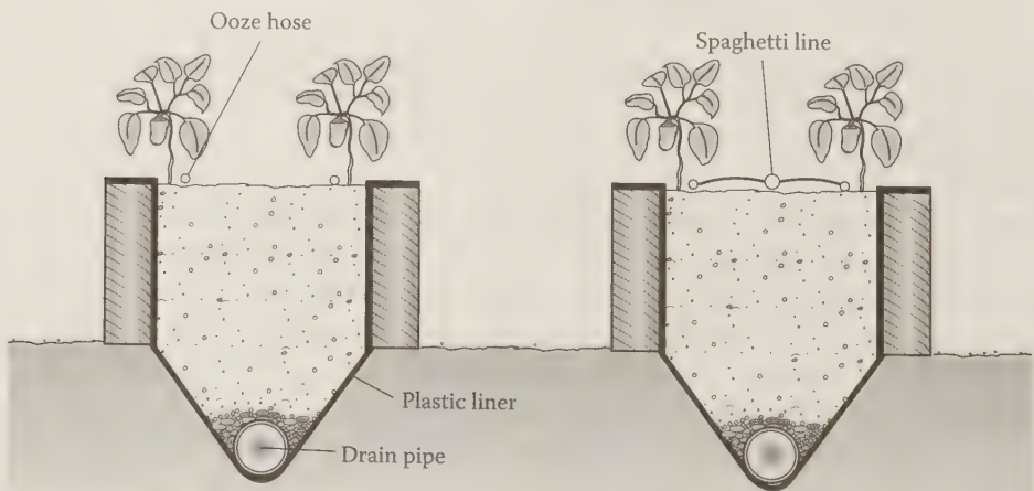
FIGURE 8.1 Cross section of sand-culture beds. (Courtesy of George Barile, Accurate Art, Inc., Holbrook, NY.)
