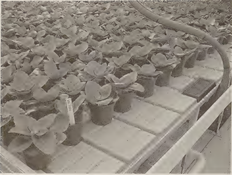
FIGURE 6.72 Fill-drain channels of ebb-and-flow bed. (From Zwart Systems, Beamsville, Ontario, Canada. With permission.)
