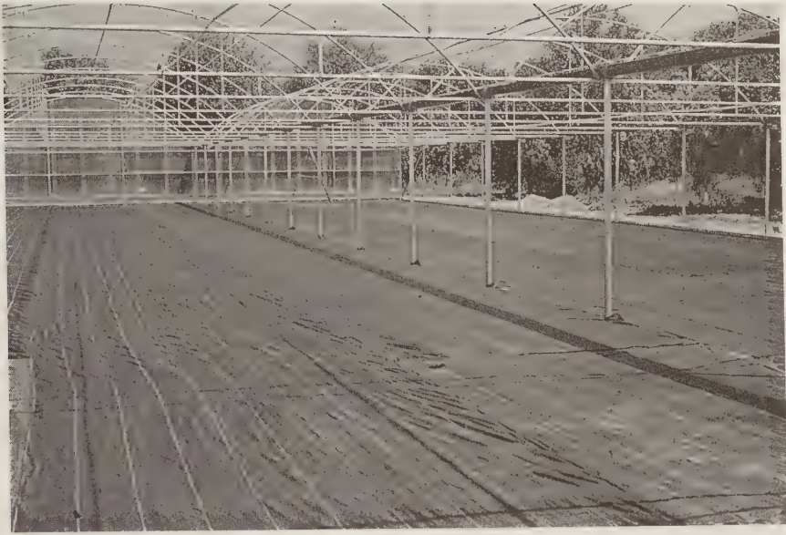
FIGURE 8.8 Greenhouse floor covered with a weed mat. (From California Watercress, Inc., Fillmore, CA. With permission.)
