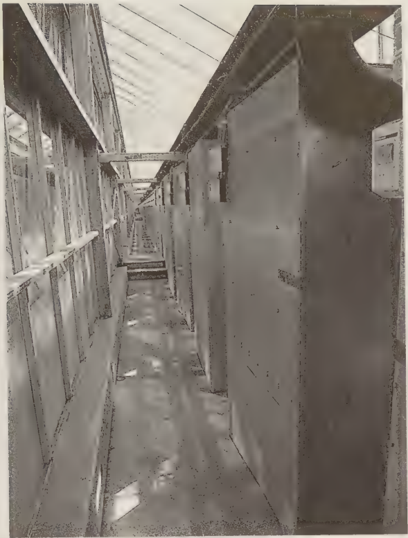
FIGURE 11.13 Cooling pad on the upper left; on the right are the heat exchangers in the fan housing. (From Houweling Nurseries Oxnard, Inc., Camarillo, CA. With permission.)
