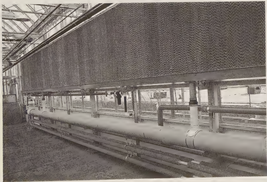
FIGURE 13.32 Evaporative cooling pad. (From Lufa Farms, Montreal, Canada. With permission.)
