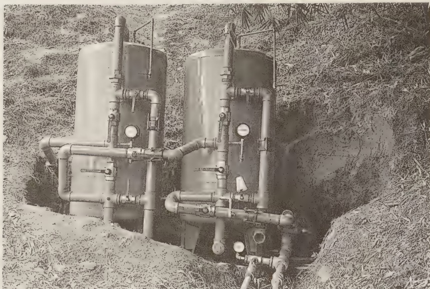
FIGURE 13.1 Filtration system of mountain spring water source. (From Hidroponias Venezolanas, S.A., Caracas, Venezuela. With permission.)
