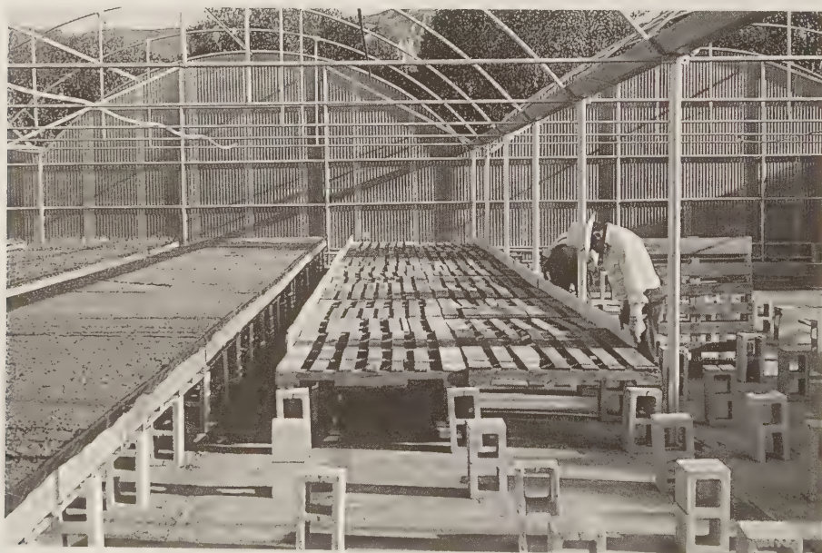
FIGURE 12.1 Beds constructed of cement blocks and pallets. (From California Watercress, Inc., Fillmore, CA. With permission.)
