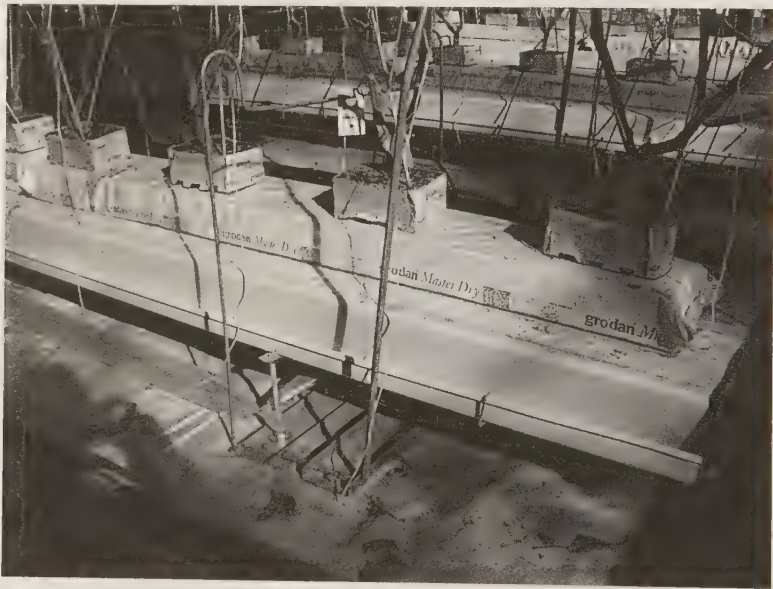
FIGURE 10.28 Wire hoops support the plant stems above the floor. Note: The slabs are set on top of FormFlex trays. The collection lip on the sides of the trays recycles the solution. (From Eurofresh Farms, Wilcox, AZ. With permission.)
