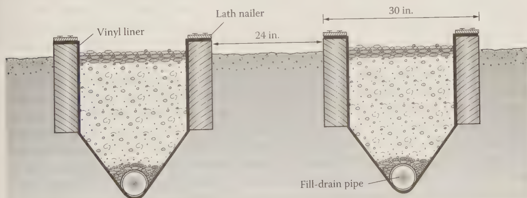
FIGURE 7.1 Cross section of a subirrigation gravel bed. (From George Barile, Accurate Art, Inc., Holbrook, NY. With permission.)
