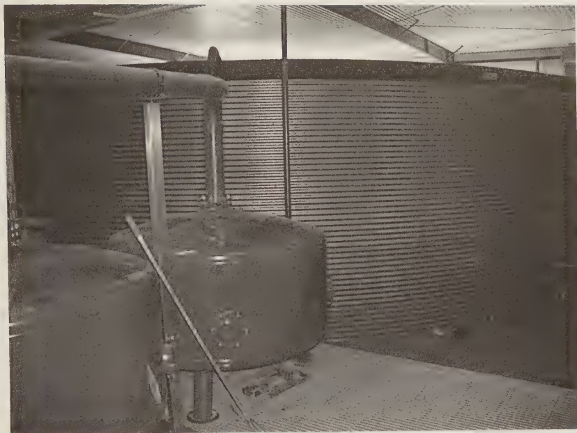
FIGURE 10.61 Sand filters with return tank. (From Eurofresh Farms, Wilcox, AZ. With permission.)
