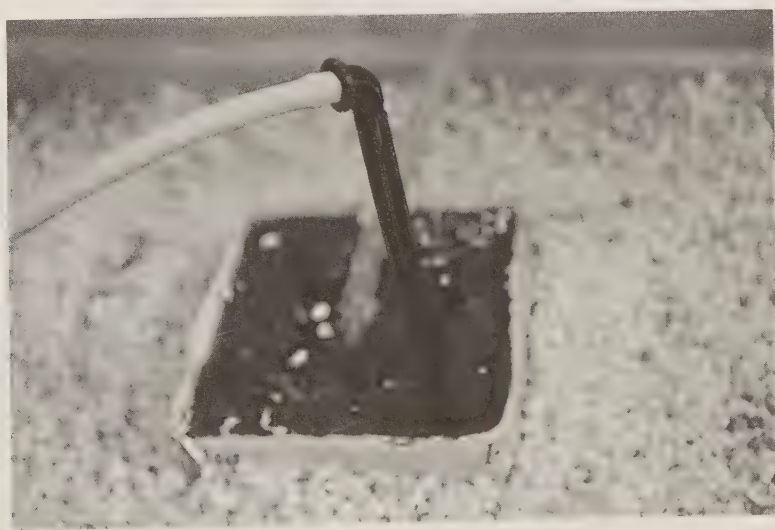
FIGURE 10.9 Drip line with ribbed stake placed at the edge of the block.
