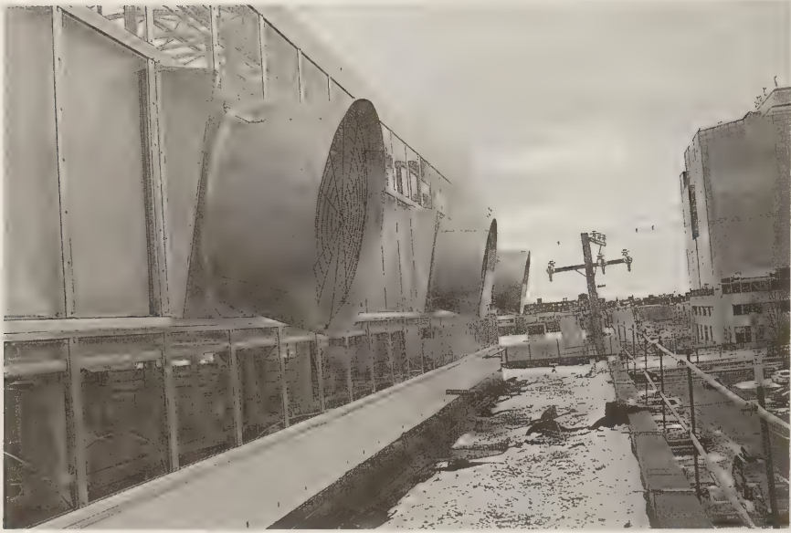
FIGURE 13.33 Exhaust fans on the side opposite to the cooling pad. (From Lufa Farms, Montreal, Canada. With permission.)
