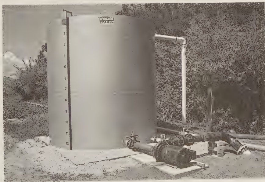
FIGURE 6.55 Booster pump pressurizes 8-in. main water line from 10,000-gal tank, which is filled from a well. (From California Watercress, Inc., Fillmore, CA. With permission.)
