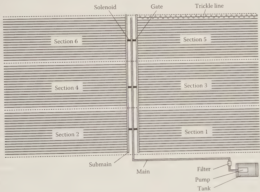
FIGURE 8.5 The installation of ooze hoses for an automated drip irrigation feeding system.
