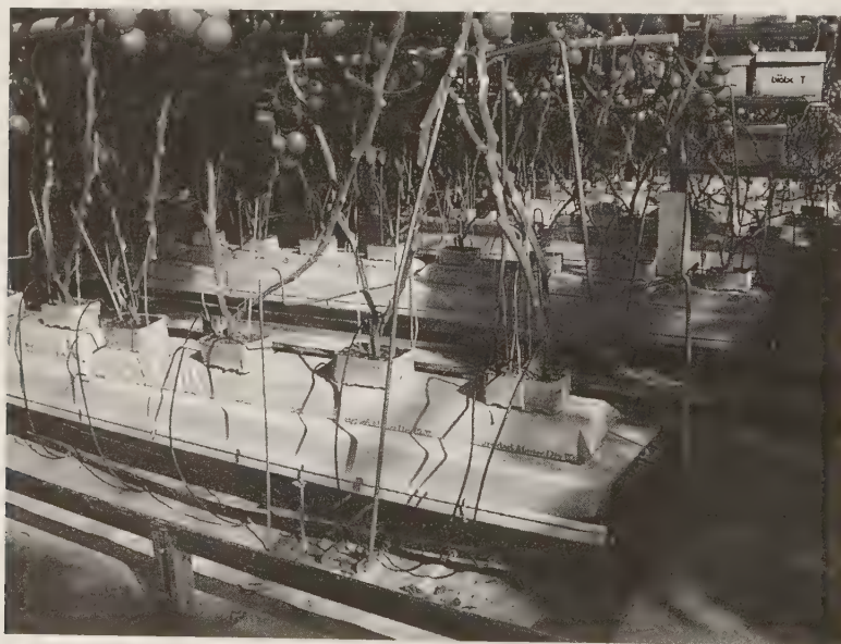
FIGURE 10.57 FormFlex "AG" gutter. (From Eurofresh Farms, Wilcox, AZ. With permission.)
