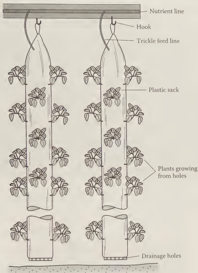
FIGURE 12.40 Schematic of hanging sack culture system. (Courtesy of George Barile, Accurate Art, Inc., Holbrook, NY.)
