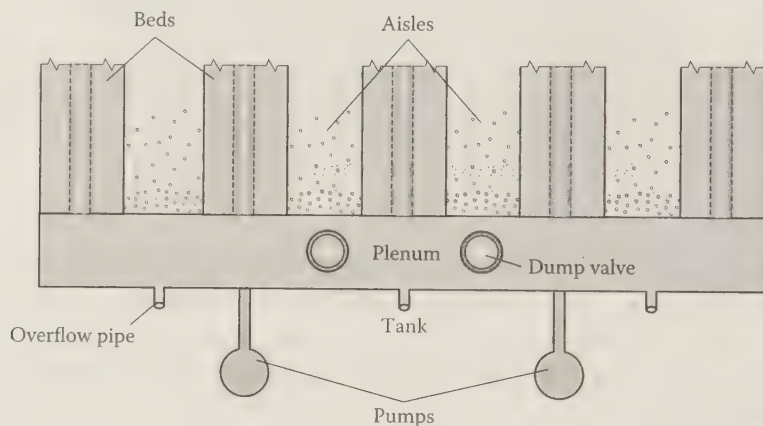
FIGURE 7.5 Plan view of plenum and nutrient tank. (Courtesy of George Barile, Accurate Art, Inc., Holbrook, NY.)
