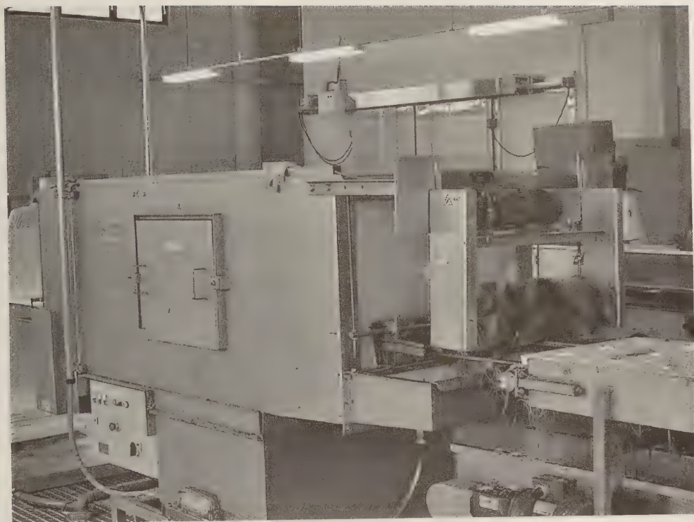
FIGURE 5.33 Board washer to clean and sterilize the boards. (From Hydronov, Inc., Japan Plantation Co. Ltd.-Nippon-Noen, Hiroshima, Japan. With permission.)
