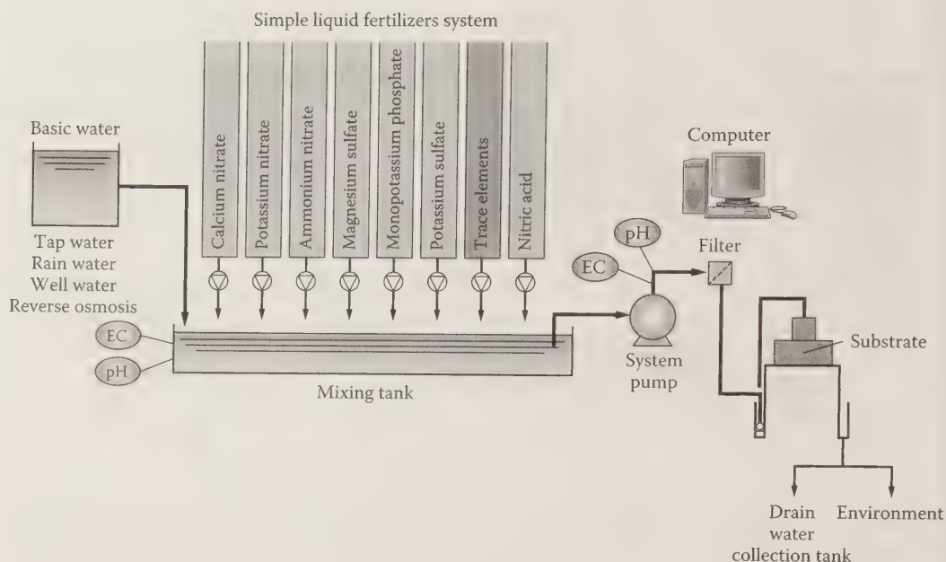
FIGURE 3.4 Individual stock mixing tank system. (Adapted from K. Welleman, The Netherlands. 6th Curso Y Congreso Internacional de Hidroponia en Mexico . Toluca, Mexico, April 17–19, 2008b. With permission. Courtesy of George Barile, Accurate Art, Inc., Holbrook, NY.)
