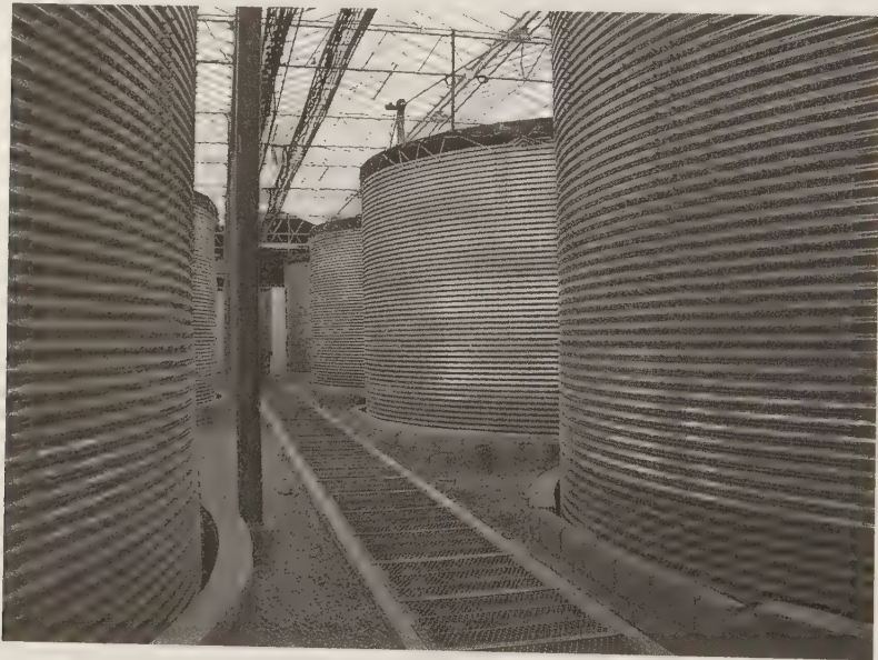
FIGURE 3.11 Large nutrient solution collection tanks in a closed system. (From Bionatur Invernaderos Biologicos De Mexico, S.A. De C.V., Jocotitlan, Mexico. With permission.)
