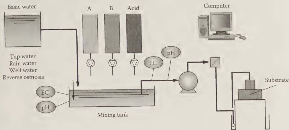
FIGURE 3.2 A, B, and acid stock mixing tank system. (Adapted from K. Welleman. 6th Curso Y Congreso Internacional de Hidroponia en Mexico . Toluca, Mexico, April 17–19, 2008b. With permission. Courtesy of George Barile, Accurate Art, Inc., Holbrook, NY.)
