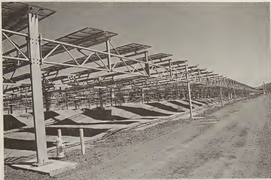
FIGURE 11.7 Four acres of solar photovoltaic system with water-retention pond below. (From Houweling Nurseries Oxnard, Inc., Camarillo, CA. With permission.)
