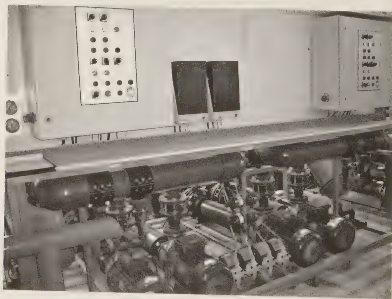
FIGURE 3.15 Fertilizer injector system. (From Bionatur Invernaderos Biologicos De Mexico, S.A. De C.V., Jocotitlan, Mexico. With permission.)
